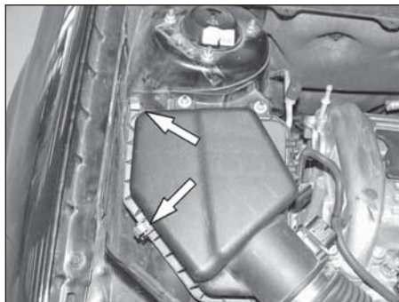
6. Unclip the air box fastening clips.
