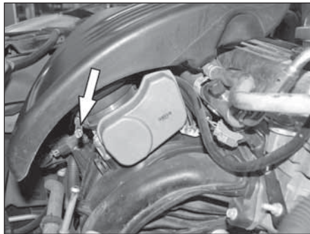
5. Loosen the hose clamp at the throttle body.
