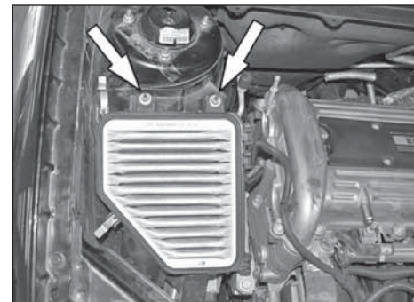
10. Loosen and remove the two air box retaining nuts then remove the air box from vehicle. NOTE: K&N Engineering, Inc., recommends that customers do not discard factory air intake.
