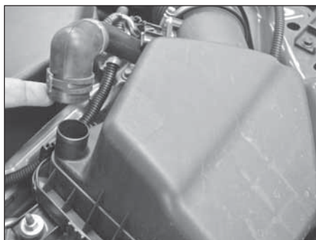
6a. On 2006 and later models, release the clamp and disconnect the air injection pump hose from the air box.
