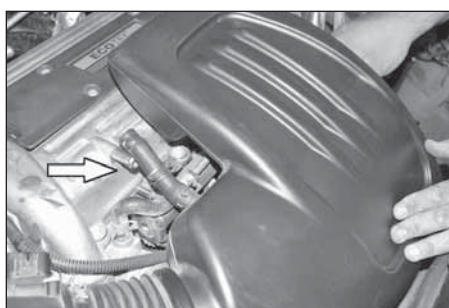
7. Release clamp and remove crankcase vent hose.
