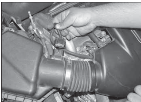
4. Disconnect the mass air sensor electrical connection.
